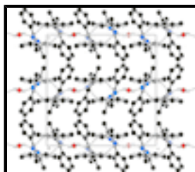
Fig. 2. The packing of the title compound, viewed down the b axis. Dashed lines indicate hydrogen bonds. H atoms not involved in hydrogen bonding have been omitted.
